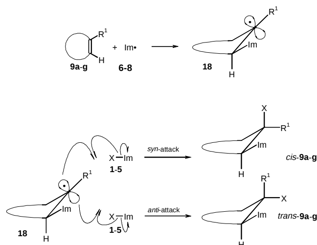
Scheme 2 The addition of imidyl radicals 1–5 to cycloalkenes 9a–g forms adduct radicals 18 . Halogen transfer by syn - or anti -attack gives the stereoisomers cis - 9a–g and trans - 9a–g .
