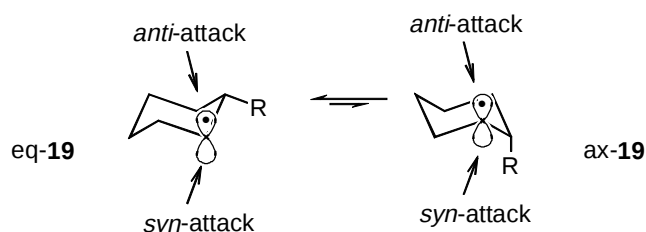
Scheme 3. The trans/cis -ratios of the products 13a–g – 17a–g are determined by the syn - or anti -attack of the N -haloimides 1–5 on the adduct radicals 19 which exist as two conformers in equilibrium, eq- 19 and ax- 19 .
